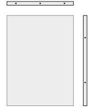
amer 710M w 701 x h 989 x d 35mm w 27,6 x h 38,94 x d 1,38" w 685 x h 981 x d 35mm w 26,97 x h 38,62 x d 1,38"
