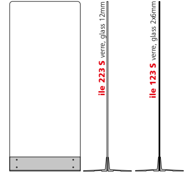
ile 223 S w 750 x h 1800 x d 512mm w 29,52 x h 70,86 x d 20,15"
